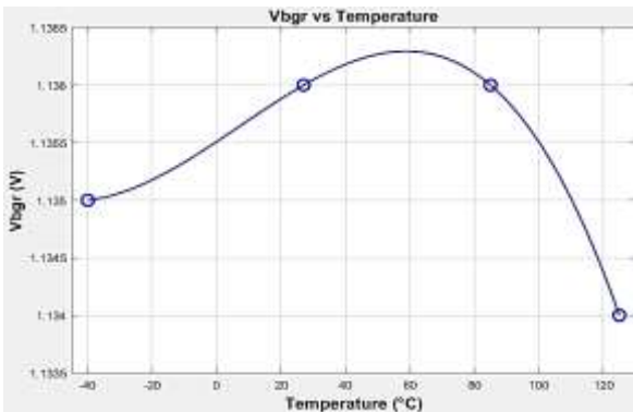
Fig. 3. First-order temperature compensation graph.
