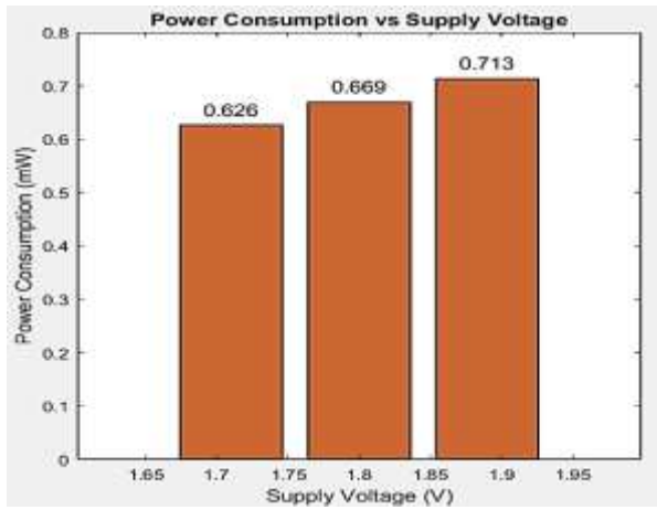
Fig. 13. Supply voltage variation effects on power.
