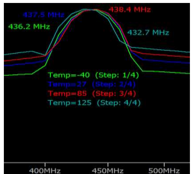
Fig. 9. Small frequency deviations of CSRO with BGR.
