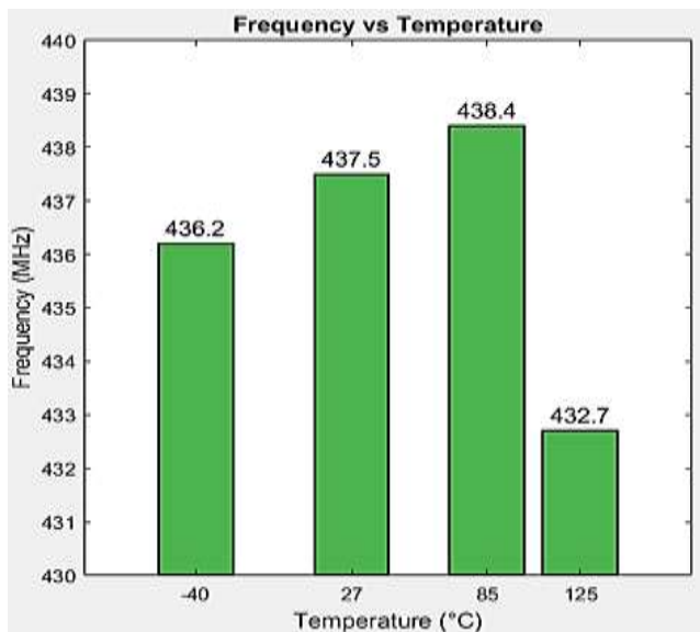
Fig. 10. Temperature variation effects on frequency.
