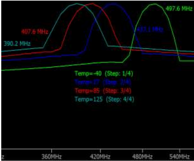
Fig. 6. Large frequency deviations of the CSRO.
