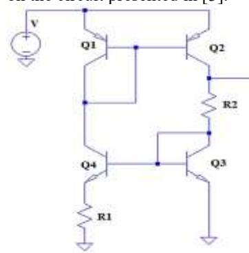
Fig. 2. Bandgap voltage reference circuit.
