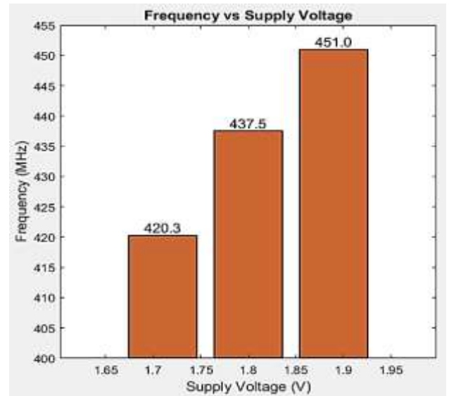
Fig. 12. Supply voltage variation effects on frequency.
