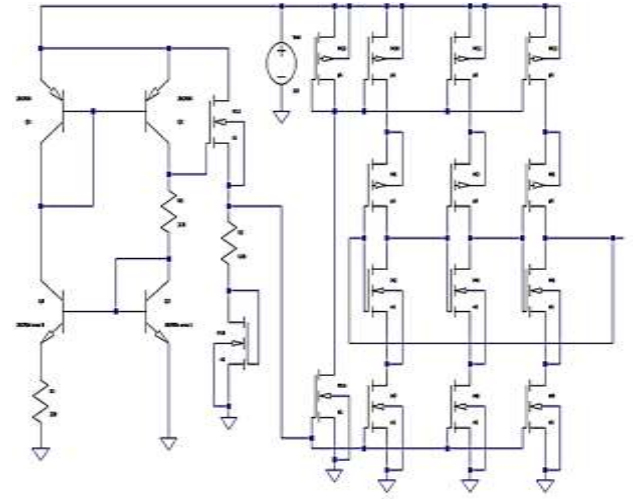
Fig. 7. The proposed CSRO with BGR.
