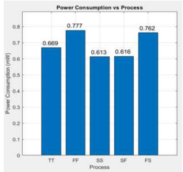
Fig. 15. Process variation effects on power.
