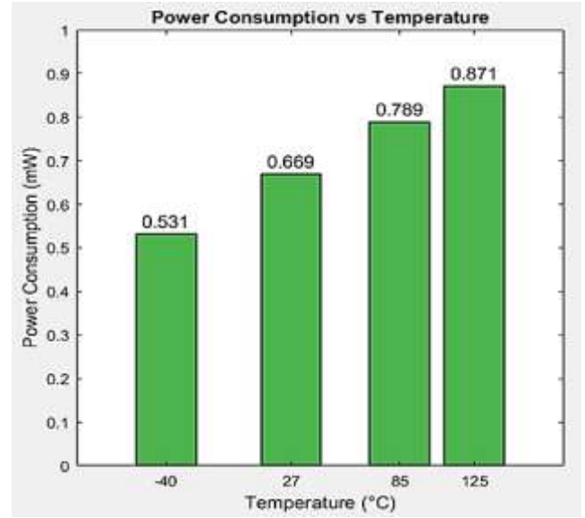
Fig. 11. Temperature variation effects on power.
