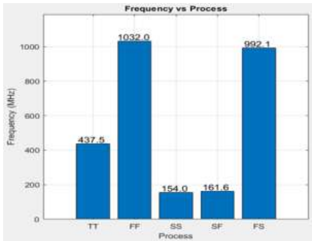
Fig. 14. Process variation effects on frequency.
