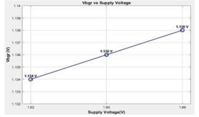
Fig. 4. Bandgap reference voltage vs supply voltage.
