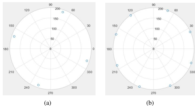
Fig. 10. Simulation Result of Polar Plot for the Beam Steered at 45°. (a) QPSK Modulation and (b) 8PSK Modulation.
