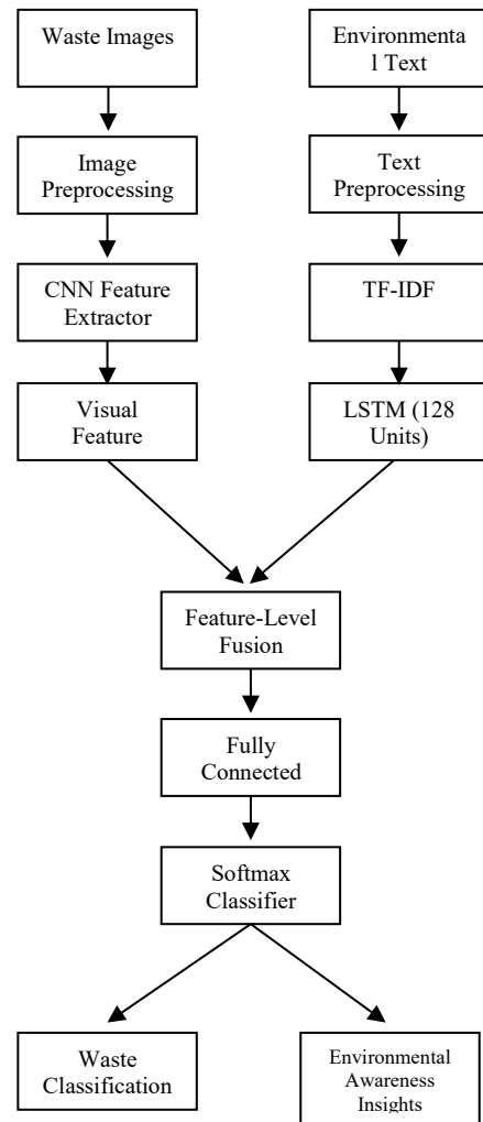
Fig. 2. Proposed multimodal deep learning framework integrating CNN-based image feature extraction and LSTM-based textual feature learning through feature-level fusion for waste classification and environmental-awareness analysis.
