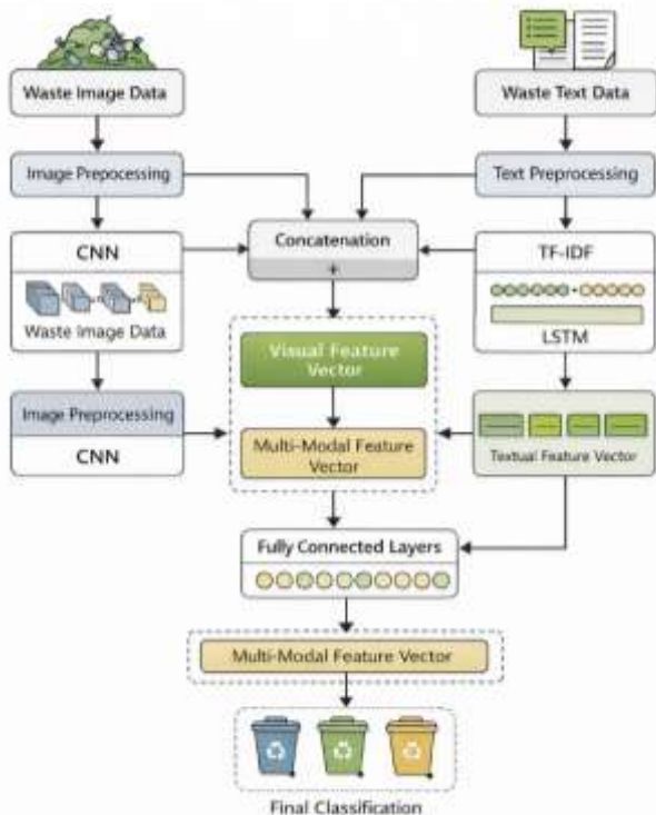
Fig. 3. Multi-modal deep learning architecture integrating CNN-based image features and LSTM-based textual features for waste classification.
